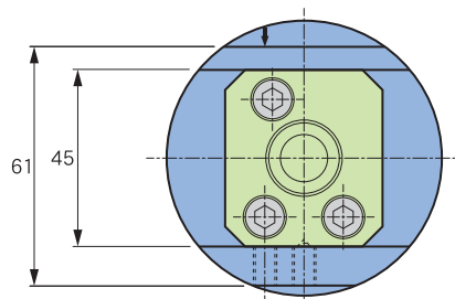
Cartridge position A
