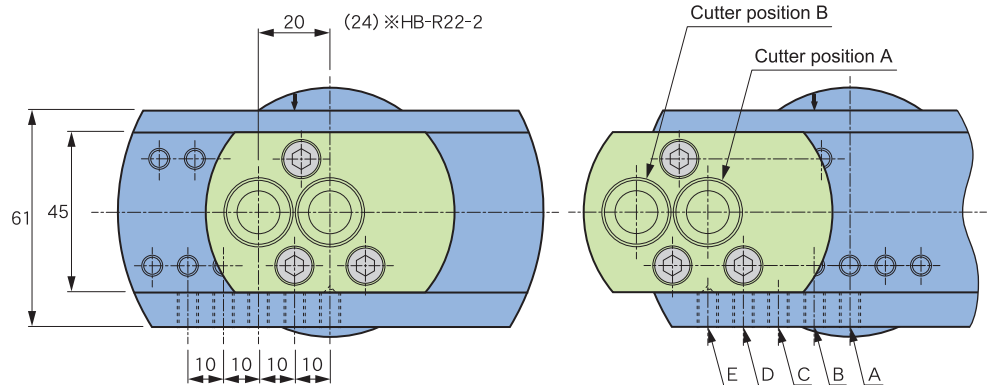
Cartridge HB-R16-2 HB-R18-2 HB-R22-2
