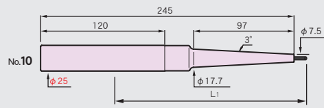
ST25-SLRA3-245-M97
