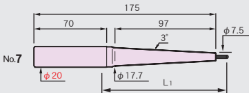
ST20-SLRA3-175-M97
