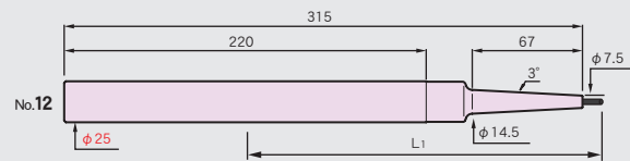
ST25-SLRA3-315-M67
